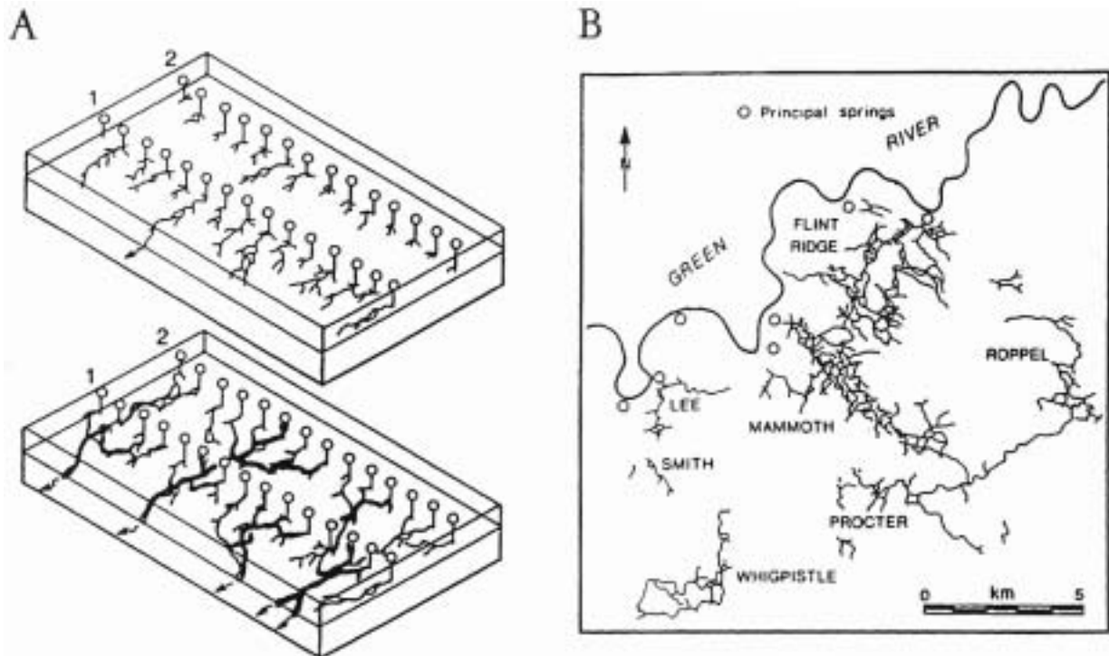
Fig. 8. (A) Patterns of proto-conduit breakthrough and connection where there are multiple ranks of inputs. (B) Map of the major galleries in Mammoth Cave and neighboring cave systems, Kentucky, to illustrate multi-rank cave genesis.
