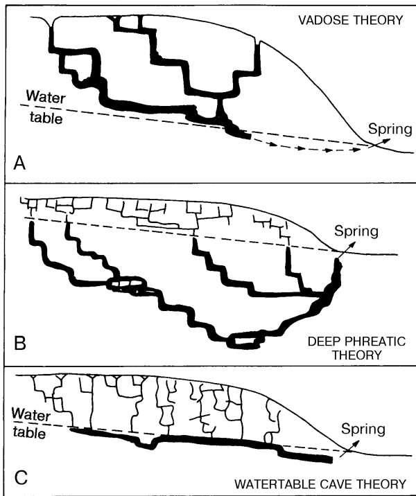
Fig. 3. Schematic diagram to depict the vadose, deep-phreatic and water-table theories of common cave genesis.
