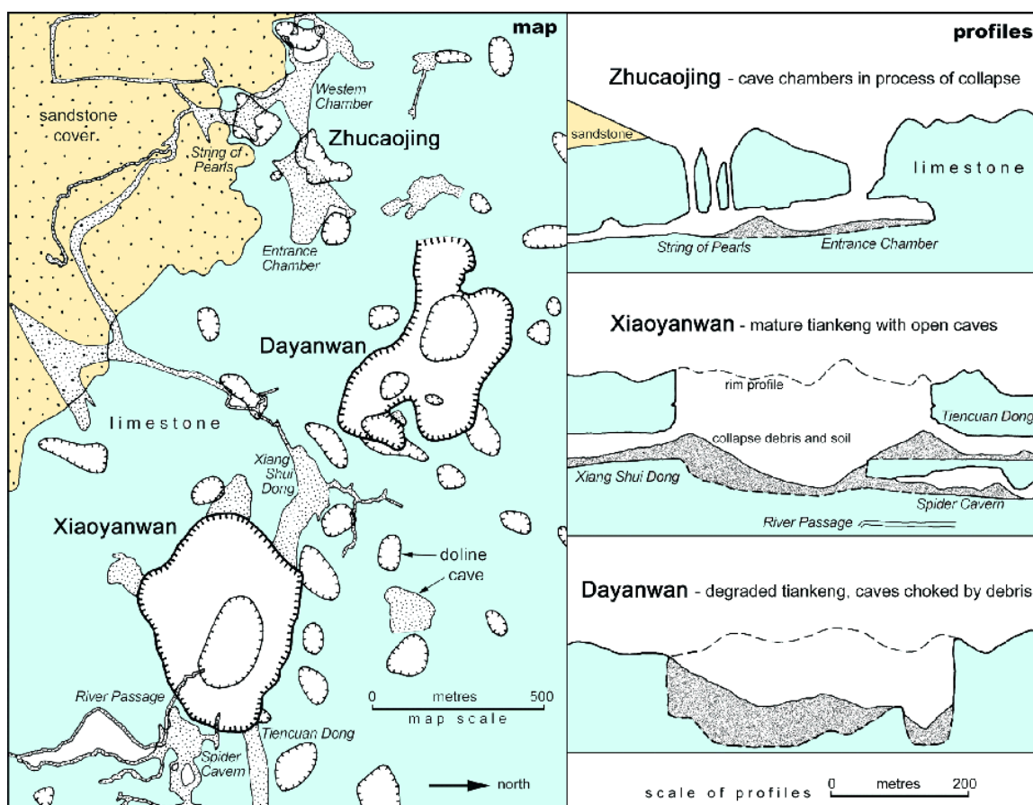
Fig. 6. Map and profiles of the three collapse sites at Xingwen, including the Xiaoyanwan tiankeng; most of the bedrock profiles are postulated as they are largely obscured by the breakdown debris.
